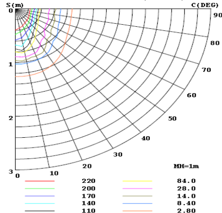
PLANAR ISOLUX DIAGRAM(UNIT:lx)
